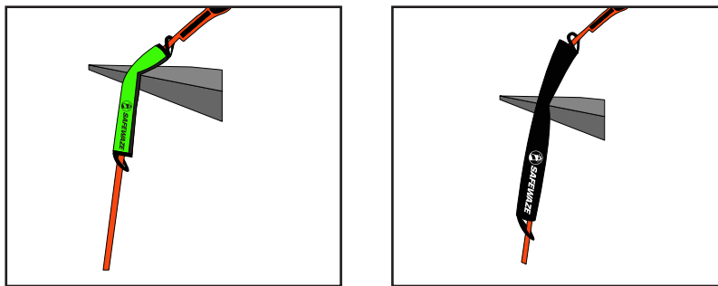
FIGURE 15 - EDGE PROTECTOR TYPICAL USE EXAMPLE
