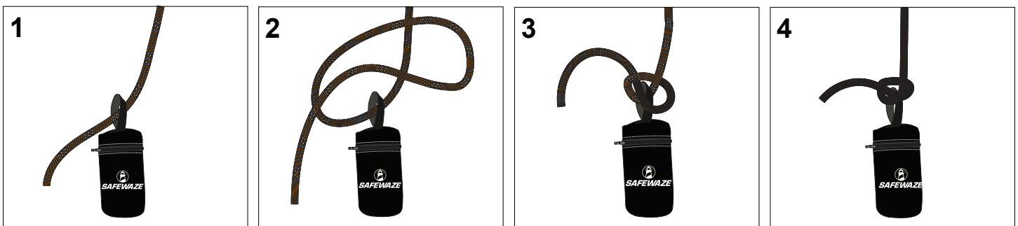
FIGURE 13 - 021-7014 ROPE COUNTERWEIGHT INSTALLATION
