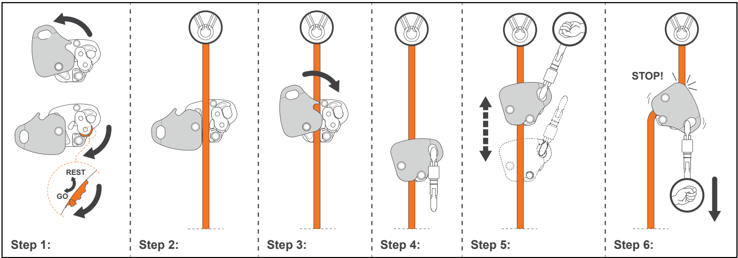
FIGURE 11 - SW-EX8000 INSTALLATION
