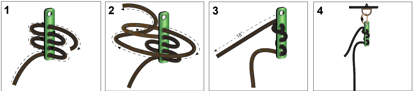
FIGURE 14 - FS875 ROPE TERMINATION PLATE INSTALLATION
