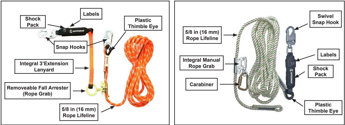
FIGURE 5 - COMPONENTS
