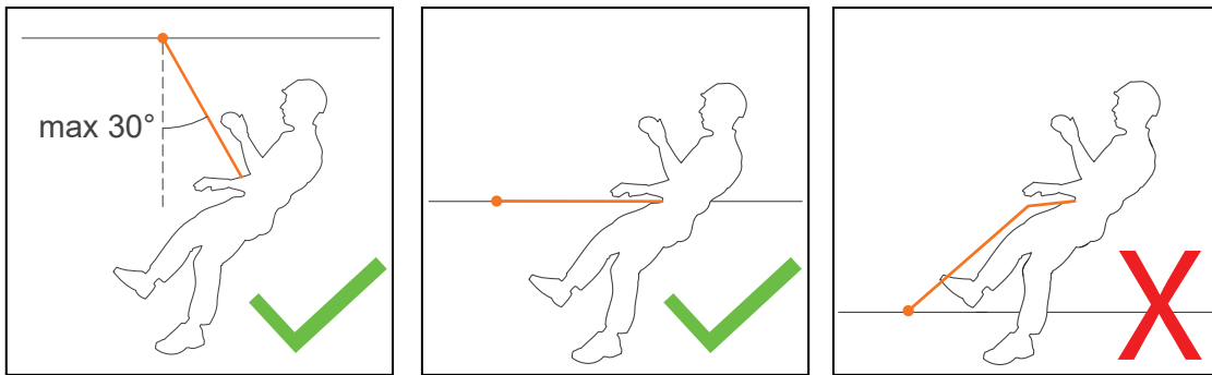
FIGURE 12 - ROPE GRAB ALLOWED ANGLE OF USE
