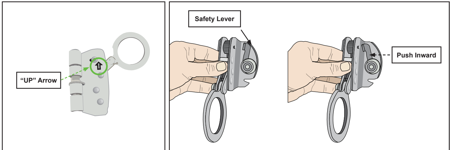
FIGURE 9 - NON-TRAILING ROPE GRAB INSTALL
