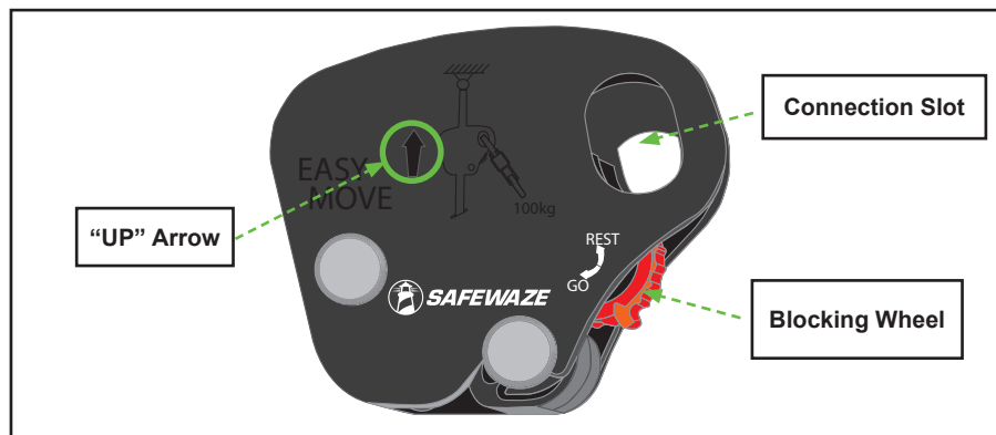
FIGURE 10 - SW-EX8000 ORIENTATION FOR INSTALL
