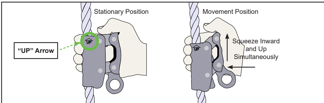
FIGURE 6- MANUAL ROPE GRAB MOVEMENT
