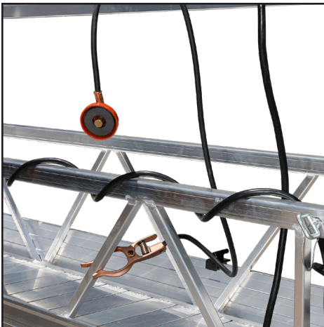
Wire Rope Insulating Tube
